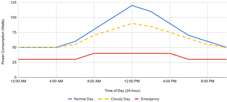
Daily Load Profile: AgroLink IoT Hub
